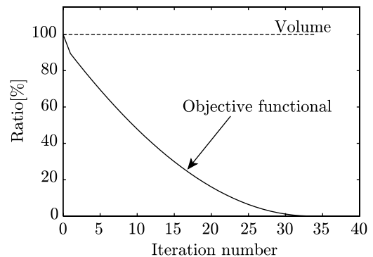
Fig. 2 Iteration history
